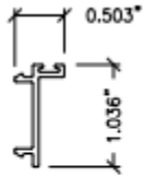
29 STILE SNAP COVER SCN-29
