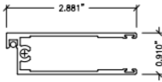
31 SCREEN RAIL SCN-31REV
