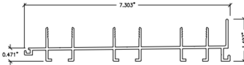
09 THREE-TRACK SILL 3TRS-9
