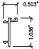
29 STILE SNAP COVER SCN-29
