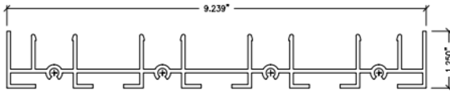
38 FOUR-TRACK JAMB 4TRJ-38
