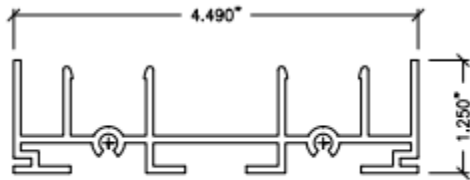
10 TWO-TRACK JAMB 2TRJ-10
