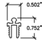
22 SNAP SCREEN GUIDE RAIL AS-22
