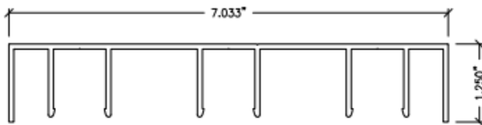
15 THREE-TRACK HEADER 3TRH-15
