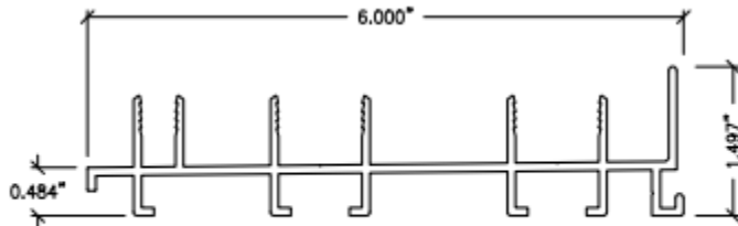
08 TWO-TRACK SILL (W/ SCREEN) 2TWS-8
