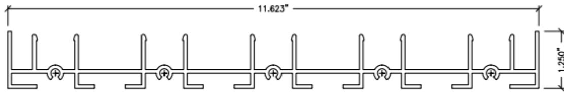
41 FIVE-TRACK JAMB 5TRJ-41
