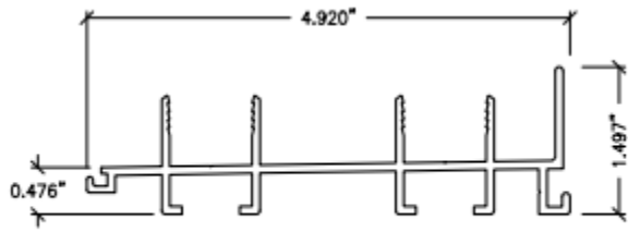
07 TWO-TRACK SILL 2TRS-7
