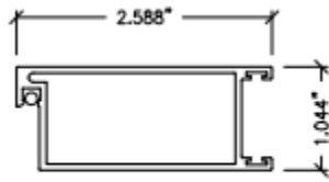
30 SCREEN STILE SCN-30
