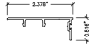
18 JAMB SNAP COVER AS-18
