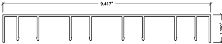
36 FOUR-TRACK HEADER 4TRH-36
