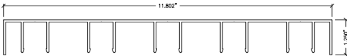
39 FIVE-TRACK HEADER 5TRH-39
