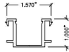
25 9/16" GLZ. STILE ADAPTER ADPT-25
