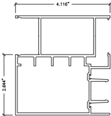
04 BUTT STILE (OFFSET) BS-4
