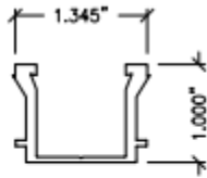
26 9/16" GLZ. RAIL ADAPTER ADPT-26
