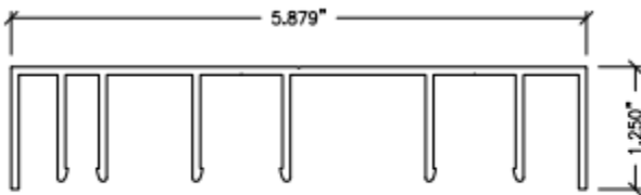
14 TWO-TRACK HEADER (W/ SCREEN) 2TRHWS-14
