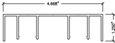
13 TWO-TRACK HEADER 2TRH-13
