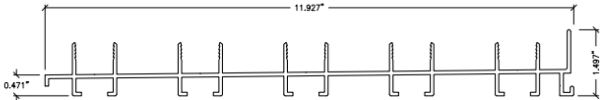
40 FIVE-TRACK SILL 5TRS-40
