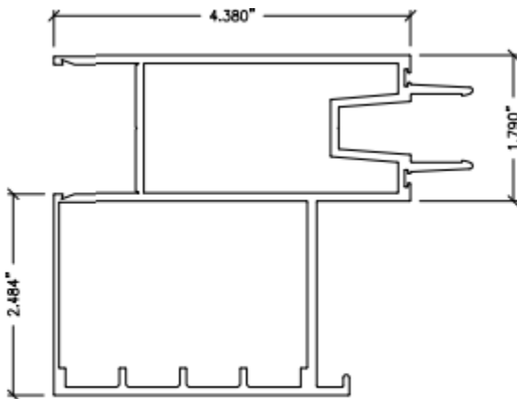
MALE BUTT STILE LIL-5
