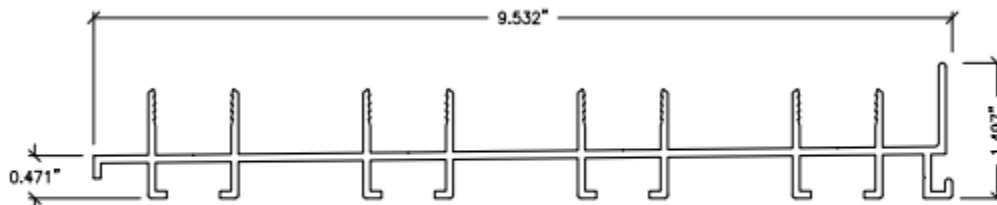
37 FOUR-TRACK SILL 4TRS-37
