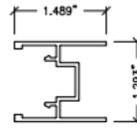
77 CENTER MEET SCREEN ADAPTER SCN-32REV
